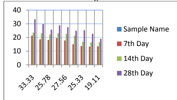
Fig. 3 Percentage Variation of Compressive Strength
