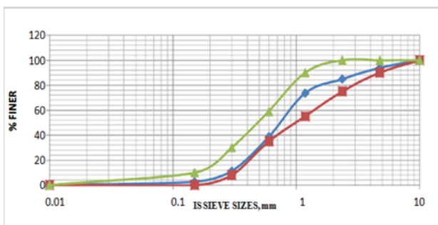
Fig 3.1 Particle size distribution for natural sand
