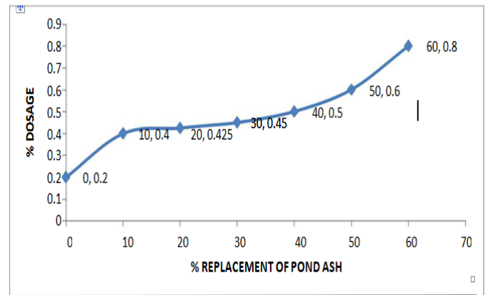
Fig 3.4 S-P Dosage for percent replacement of Pond ash
