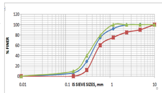
Fig 3.2 Particle size Distribution of Pond ash
