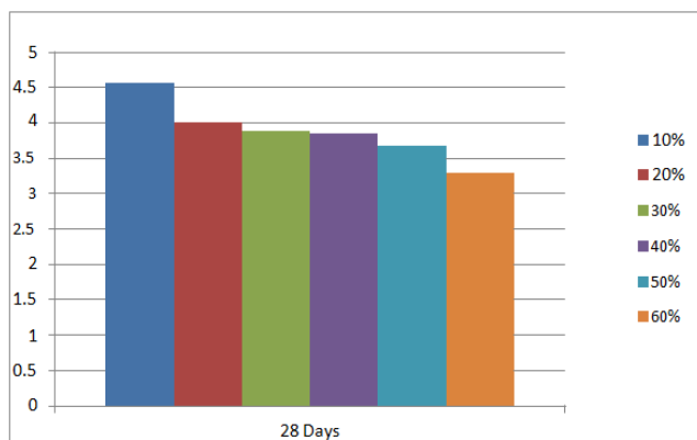
Fig 4.2 Flexural Strength Vs % Pond ash replacement
