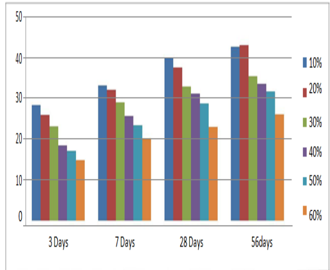
Fig 4.1 Compressive Strength V/s % Pond ash replacement
