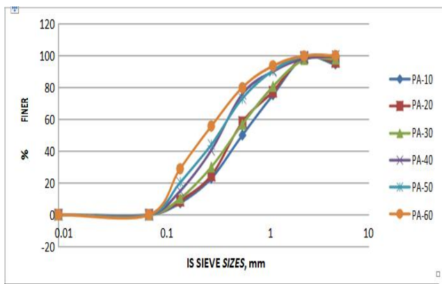
Fig 3.3 Particle Size Distribution of mixed Fine aggregate
