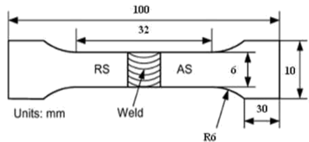
Figure 7. Dimensions of tensile specimen as per ASTM E8 Standard
